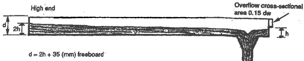
FIGURE 4.3.1 OVERFLOW OUTLET
