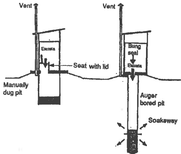
FIGURE 4.2 DRY (NONFLUSH) PIT LATRINES
