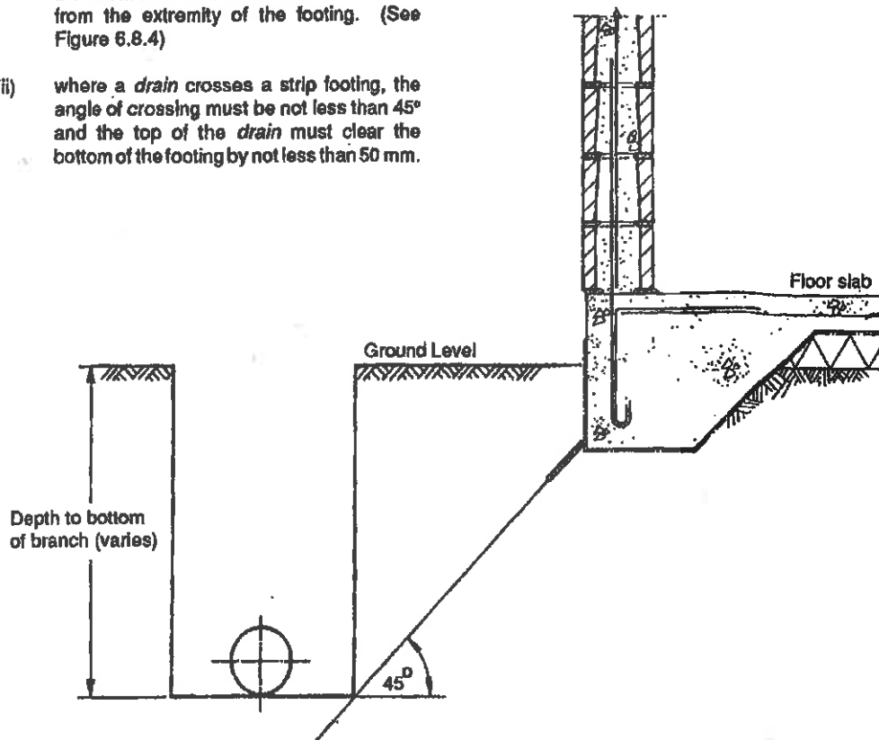
FIGURE DF6.8.4
